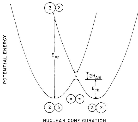
Figure 1. Plot of the potential energy of the reactants (precursor complex) and products (successor complex) as a function of nuclear configuration for an electron-exchange reaction. E_{\text{th}} is the barrier for the thermal electron transfer, E_{\text{op}} is the energy for the light-induced electron transfer, and the splitting at the intersection of the surfaces is equal to 2H_{\text{AB}} where H_{\text{AB}} is the electronic coupling matrix element. Note that H_{\text{AB}} \ll E_{\text{th}} in the weak interaction model. The circles indicate the relative nuclear configurations of the two reactants of charges 2+ and 3+ in the precursor complex, the optically excited precursor complex, the activated complex, and the successor complex.
